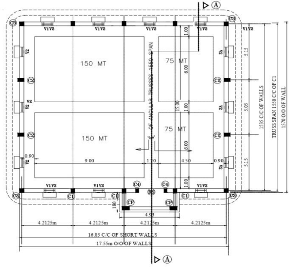
PLAN FOR (450 MT) WH. BLDG.
